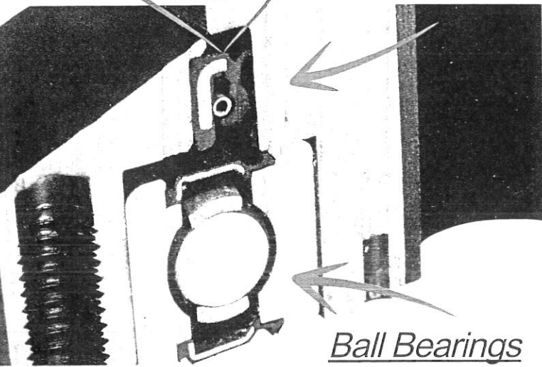
ALUMINUM DRIVER PLATE WITH THROUGH HOLE
